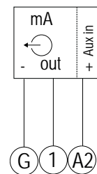
Fig. 19 Analog current input, 3 wires (product code: 2TCW)
